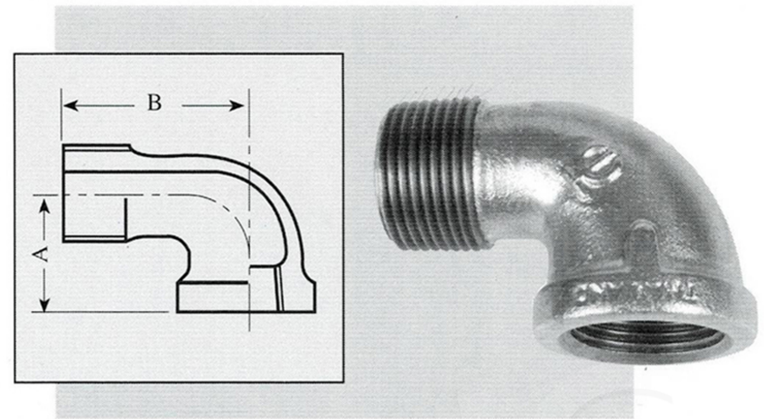
FIG. 132 Street Elbows, Banded, Equal (SL)
